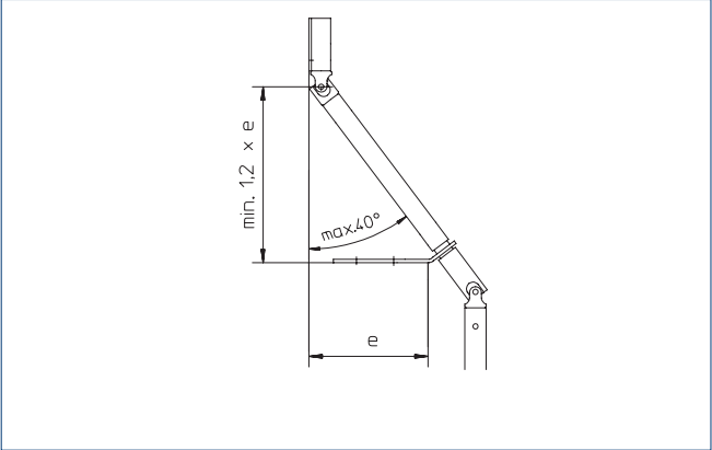
Swivel joint fixed crank rod | e = reveal depth
